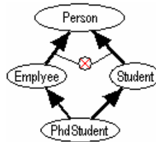
Fig. 1. Unsatisfiability of ORM schema.
